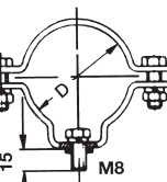
Pipe Clamp
